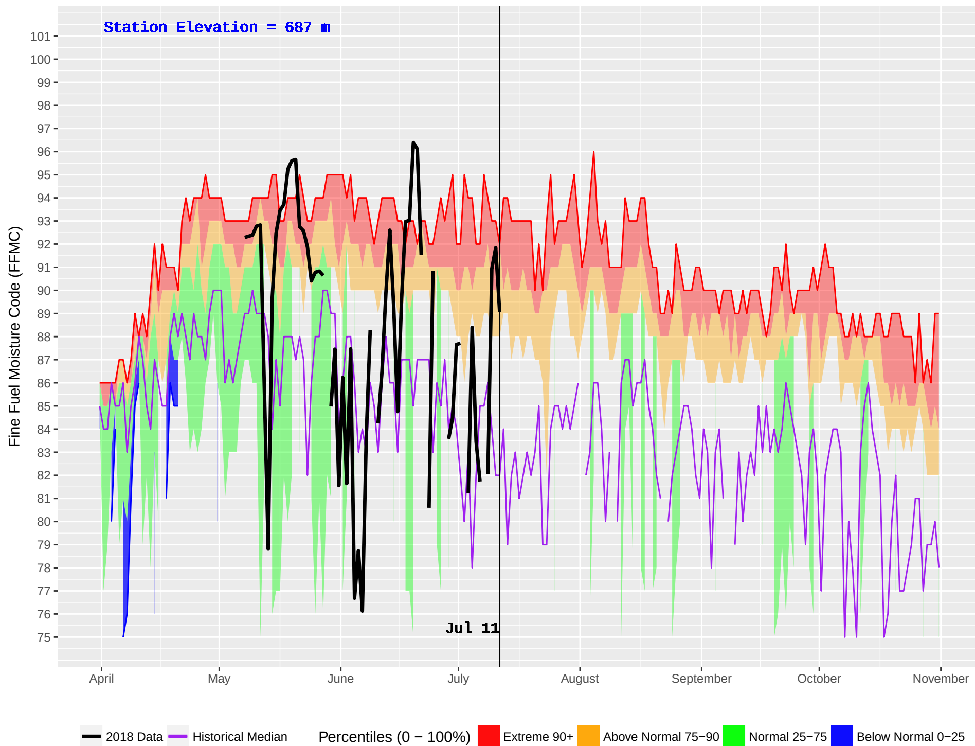
KETCHIKA (444) : Historical (1986–2016) and Current (2018) Noon Fine Fuel Moisture Code (FFMC)
