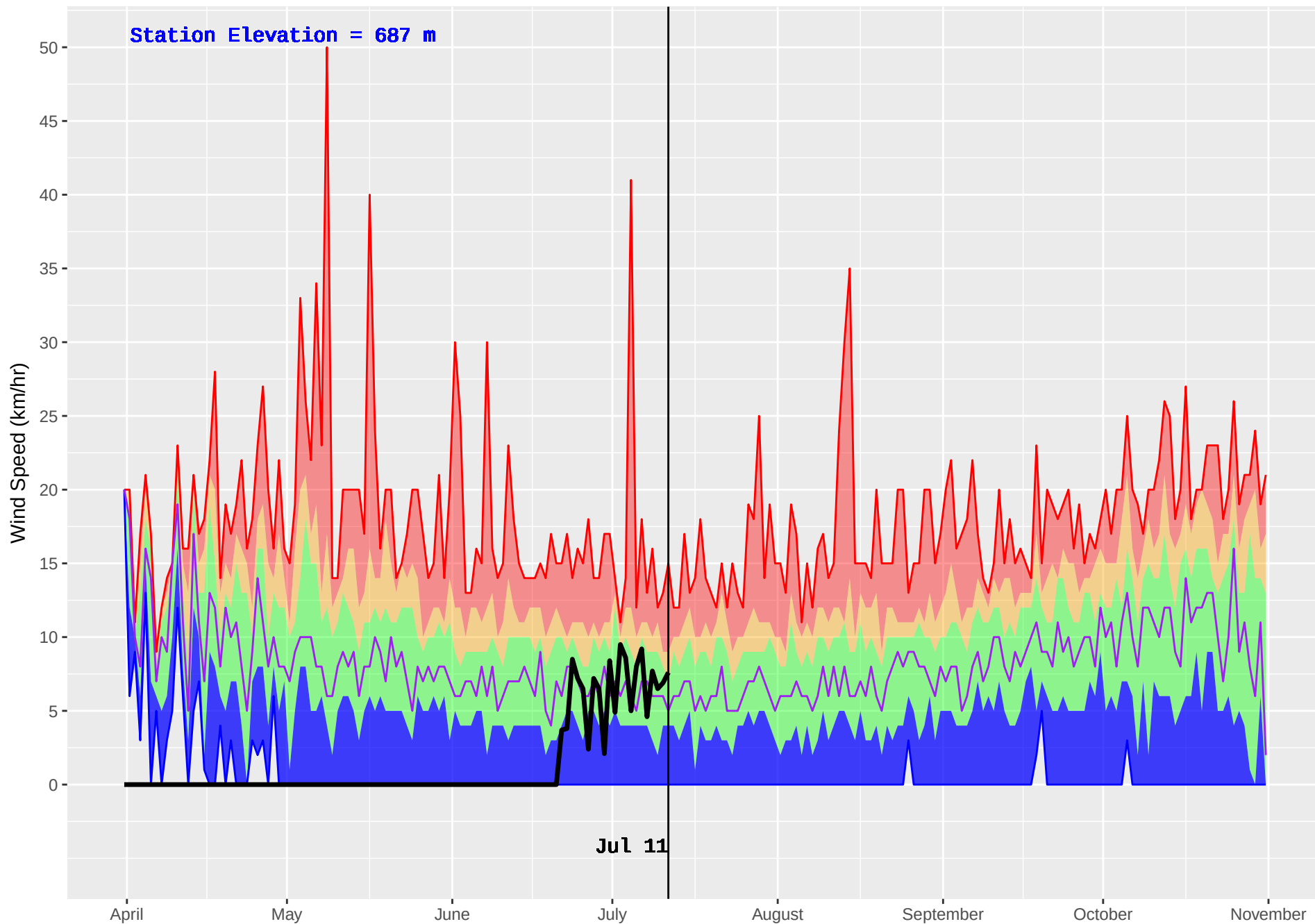
KETCHIKA (444) : Historical (1986–2016) and Current (2018) Noon Wind Speed
